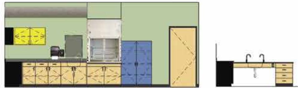
EAST ELEVATION / STUDENT WORKSTATION ELEVATION
